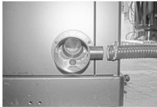
Attaching hose to dust port:
