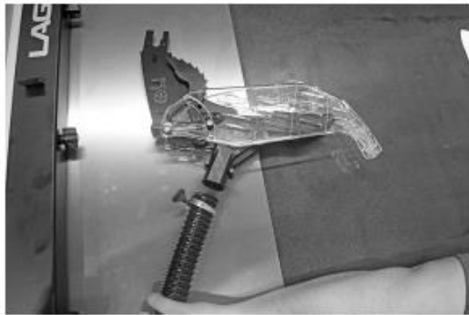
Attaching hose to blade guard assembly:
