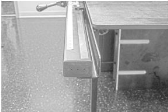
Front guide rail seated on front rail:
